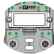
M12 D-coded, Modbus TCP/IP Port 1/2 接线示意
