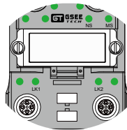
M12 D-coded, PROFINET Port 1/2 接线示意
