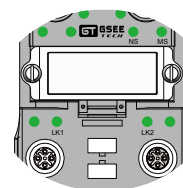
M12 A-coded, DeviceNET Port 1/2 接线示意
